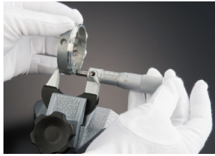
Ratchet stop 102-301
